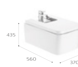
Square wall-hung bidet
