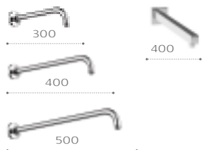
5B0150C00 Wall arm 300mm 5B0250C00 Wall arm 400mm 5B0350C00 Wall arm 500mm 5B0950C00 Square wall arm 400mm
